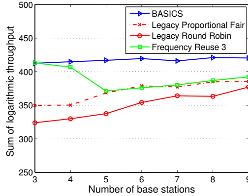
Figure 3.6: Performance comparison with a fixed number of users (150 users).
