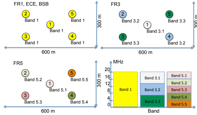
Figure 6.3: Network scenario with 5 base stations placed at regularly spaced positions, and 750 users (not shown in the figure) randomly dropped into an area of 600 m \times 300 m. For each tested scheme, the figure reports the BS baseband bandwidth.
