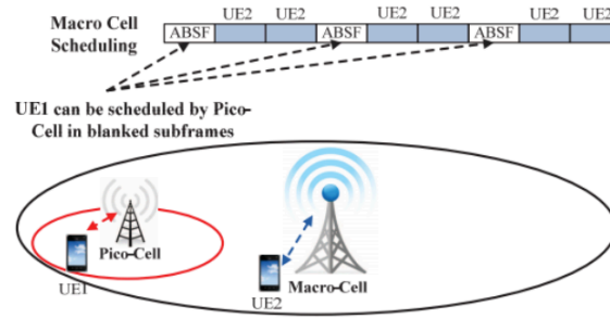
Figure 1.2: Almost Blank SubFrame (ABSF) explanation scheme [88].
