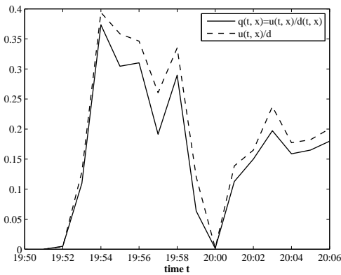
Fig. 3. q(t, x) ratio and u(t, x)/d , upload rate normalized to the streaming rate d = 224 kbit/s, during the first connection minutes
