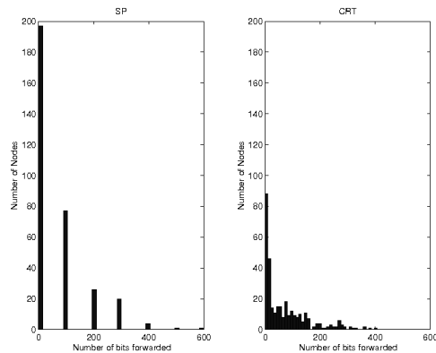
Fig. 8. Number of bits forwarded from nodes belonging to CL_{ID} = 2 , when GridSize = [300m \times 300m] , w = 100 bits and \rho = 0.03 .
