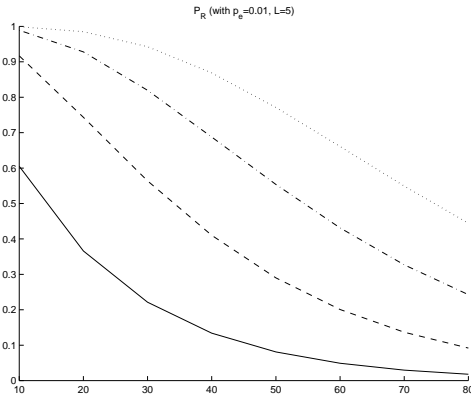
Fig. 4. Reliability function: p_e = 10^{-2} , L = 5 , f \in \{0, \dots, 3\} .
