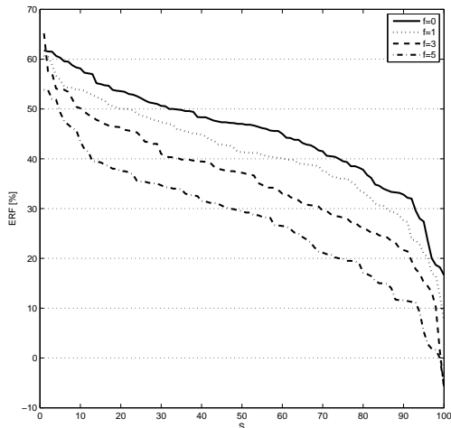
Fig. 6. ERF vs. sorted topologies, S, with different values of f .
