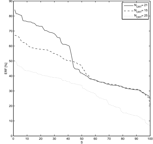
Fig. 5. ERF vs. sorted topologies, S , with different values of N_{CRT} .
